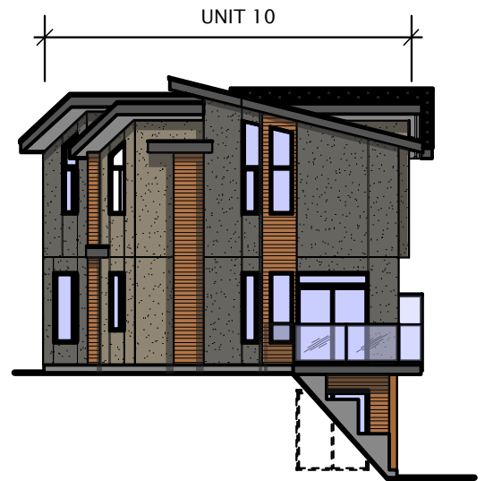
LEFT ELEVATION
