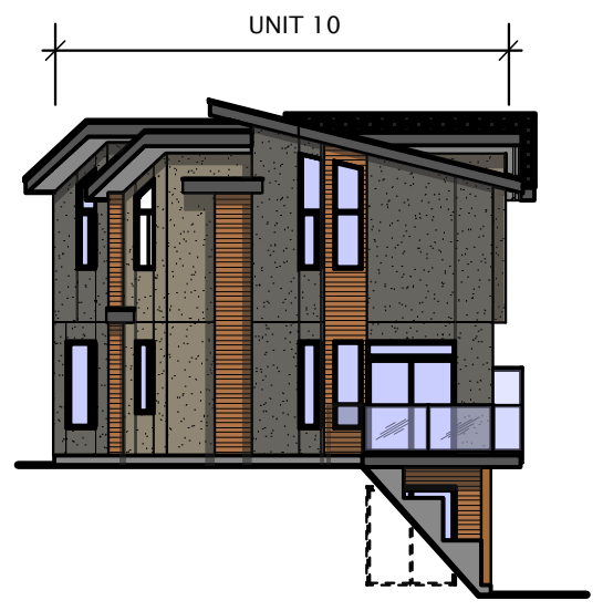
LEFT ELEVATION
